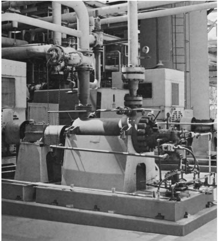
Photo: Two Type CEUHS CECON clutches at large Texas refinery used with hydraulic turbines to recover energy from process fluid
